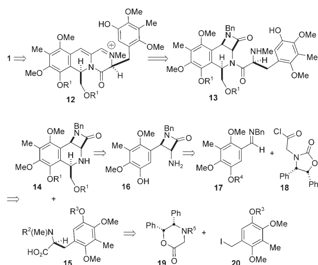
Scheme 3. Retrosynthetic analysis of 1 . Bn = benzyl.
