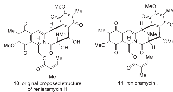
Scheme 2. The structures of cribrostatin 4 (renieramycin H) and renieramycin I.
